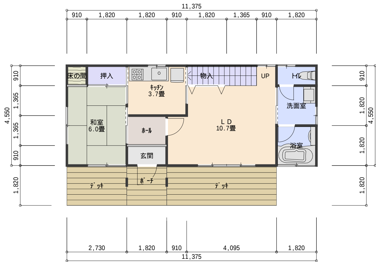
1F
